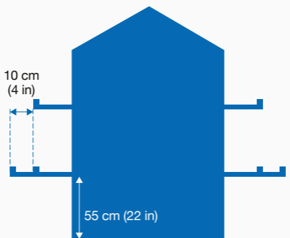
Manual nest box set-up.
