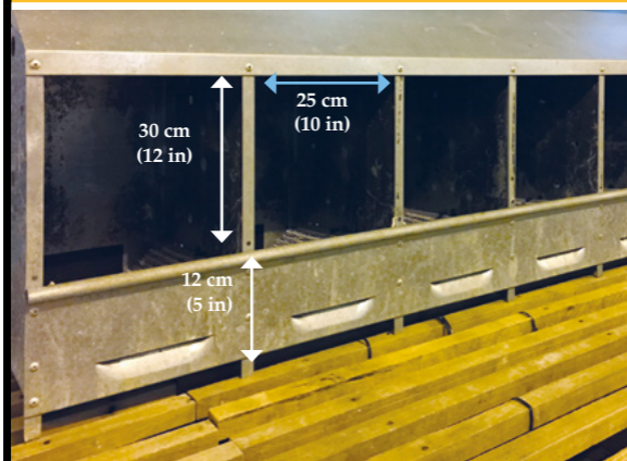
Nest box entrance dimensions.
